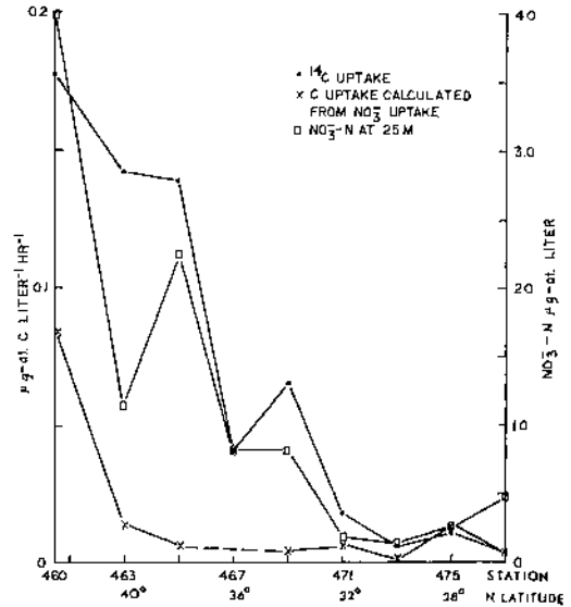
FIG. 6. Comparison of primary productivity measured on Chain cruise 25 by the ^{14}\text{C} method and new productivity measured by the ^{15}\text{N} method.
