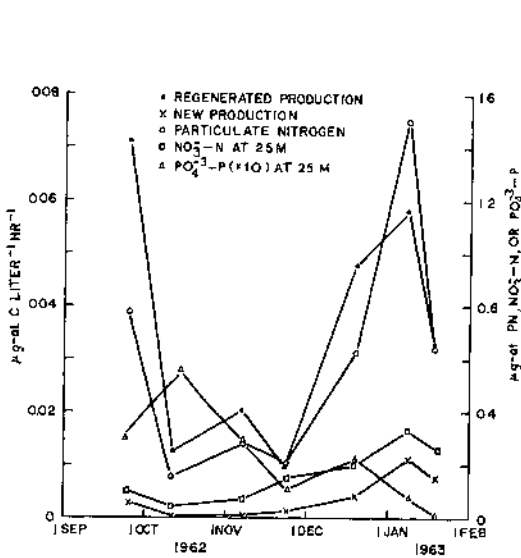
FIG. 5. Seasonal changes in nitrogen uptake at station S near Bermuda expressed in terms of carbon as new and regenerated primary productivity.
