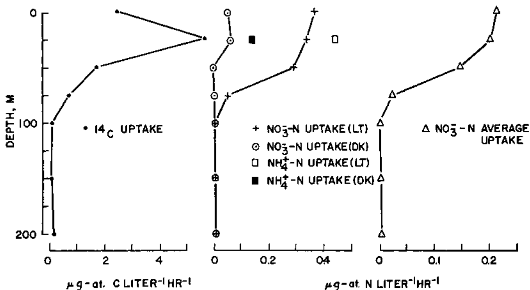
FIG. 3. Uptake of ^{15}\text{N} -labeled \text{NO}_3^- and ^{14}\text{C} at station 5 of cruise 2 of the RV Atlantis II in vertical series.
