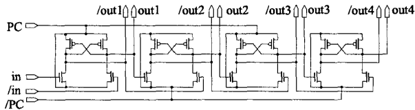
Fig. 2. A 4-stage cascade of PAL inverters
