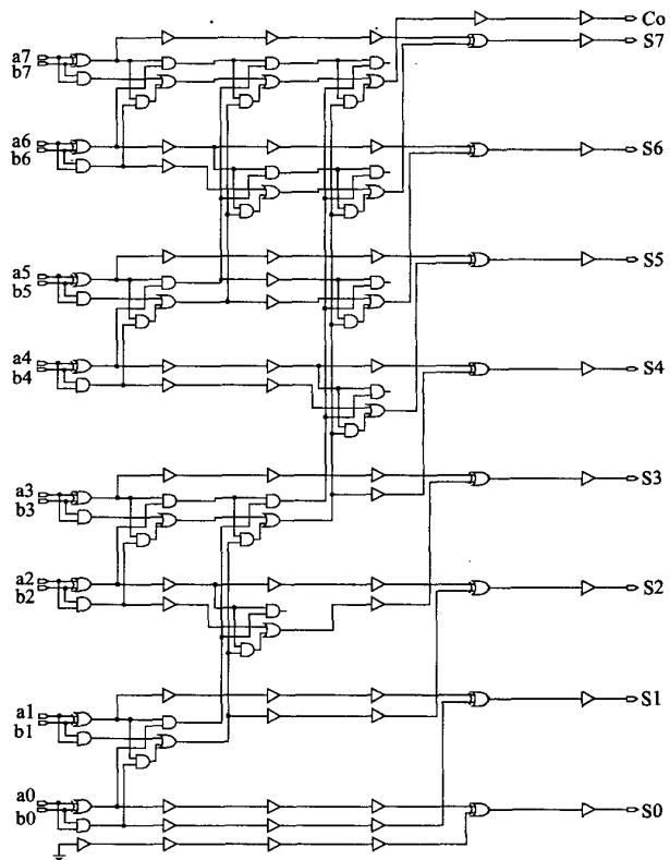
Fig. 4. Schematic diagram of 8-bit CLA
