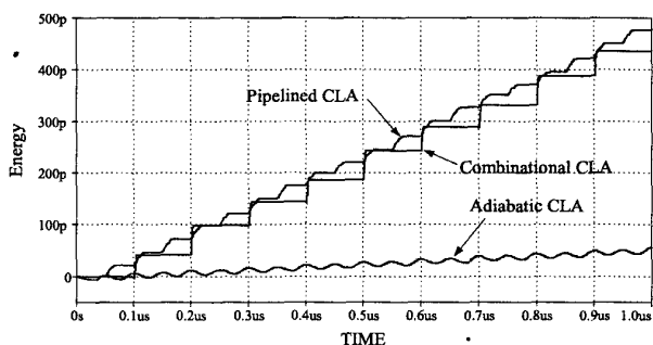
Fig. 8. Energy profiles
