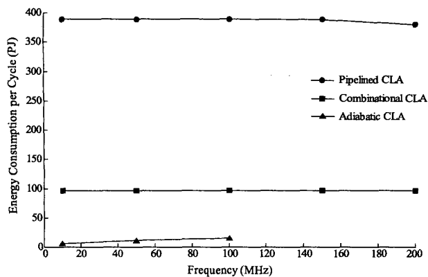
Fig. 7. Energy consumption vs. frequency at constant 3.3V supply voltage
