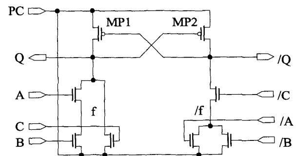
Fig. 1. Implementation of Q=A \cdot B+C in PAL
