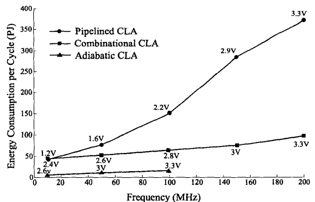
Fig. 6. Energy consumption vs. frequency
