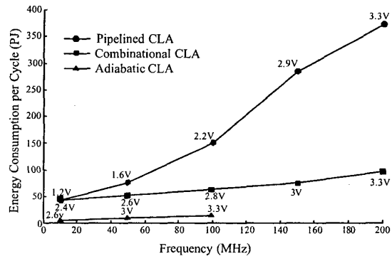
Fig. 6. Energy consumption vs. frequency
