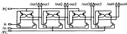
Fig. 2. A 4-stage cascade of PAL inverters
