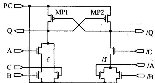
Fig. 1. Implementation of Q=A \cdot B+C in PAL
