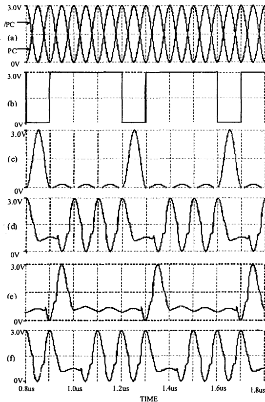
Fig. 3. Waveforms obtained from HSPICE simulations of a 4-stage pipeline of PAL inverters. (a) power clock (PC and /PC), (b) input of 1 st stage, (c) output of 1 st stage, (d) output of 2 nd stage, (e) output of 3 rd stage, and (f) output of 4 th stage.
