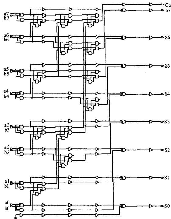
Fig. 4. Schematic diagram of 8-bit CLA
