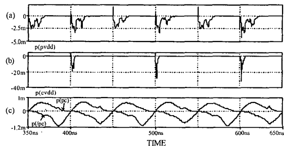
Fig. 7. Power profiles of CLAs (a) Pipeline (b) Combinational (c) Adiabatic
