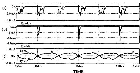
Fig. 9. Switching current waveforms of CLAS (a) Pipeline (b) Combinational (c) Adiabatic
