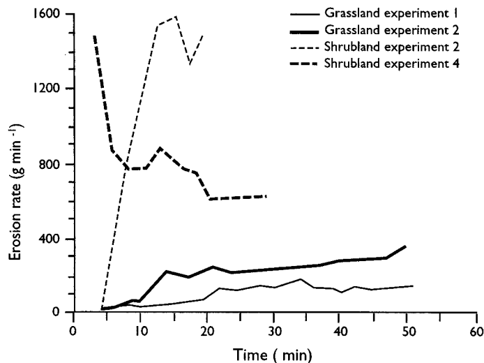
Figure 9. Comparison of the overall erosion rates in the large plot experiments on the shrubland and grassland at Walnut Gulch (redrawn after Parsons et al. , 1996a. Modified and reprinted from Geomorphology , 14, Parsons AJ, Abrahams AD, Wainwright J, 'Responses of interrill runoff and erosion rates to vegetation change in southern Arizona', 311–317, 1996, with permission from Elsevier Science.)
