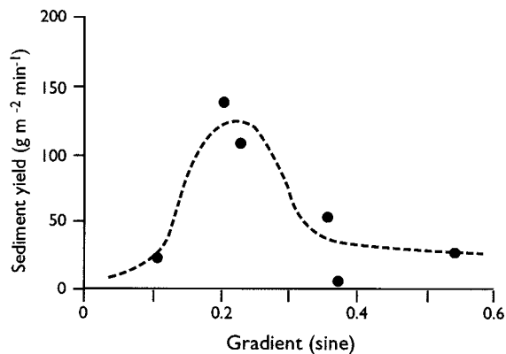
Figure 7. Relationship between sediment yield and slope gradient for a series of small-plot experiments on shrubland sites at Walnut Gulch (redrawn after Abrahams et al. , 1988a. Modified and reprinted from Catena , 15, Abrahams AO, Parsons AJ, Luk S-H, 'Hydrologic and sediment responses to simulated rainfall on desert hillslopes in southern Arizona', 103–117, 1988, with permission from Elsevier Science.)
