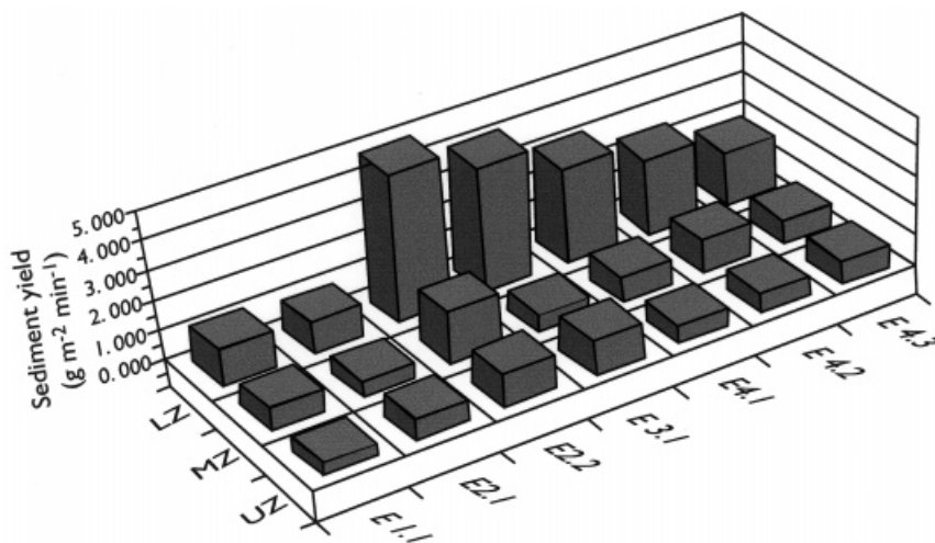
Figure 10. Rill erosion rates derived from repeated cross-sectional surveys during the large shrubland plot experiment at Walnut Gulch (redrawn after Luk et al. , 1993. Modified and reprinted from Catena , 20 , Luk S-H, Abrahams AD, Parsons AJ, 'Sediment sources and sediment transport by rill flow and interrill flow on a semi-arid piedmont hillslope, southern Arizona', 93–111, 1993, with permission from Elsevier Science.)
