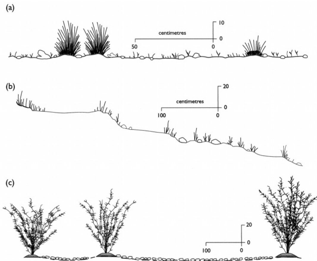
Figure 5. Microtopography of the Walnut Gulch grassland and shrubland sites defined by surveys carried out at 1-cm intervals (redrawn after Parsons et al. , 1996a. Reproduced by permission of John Wiley & Sons, Ltd.)
