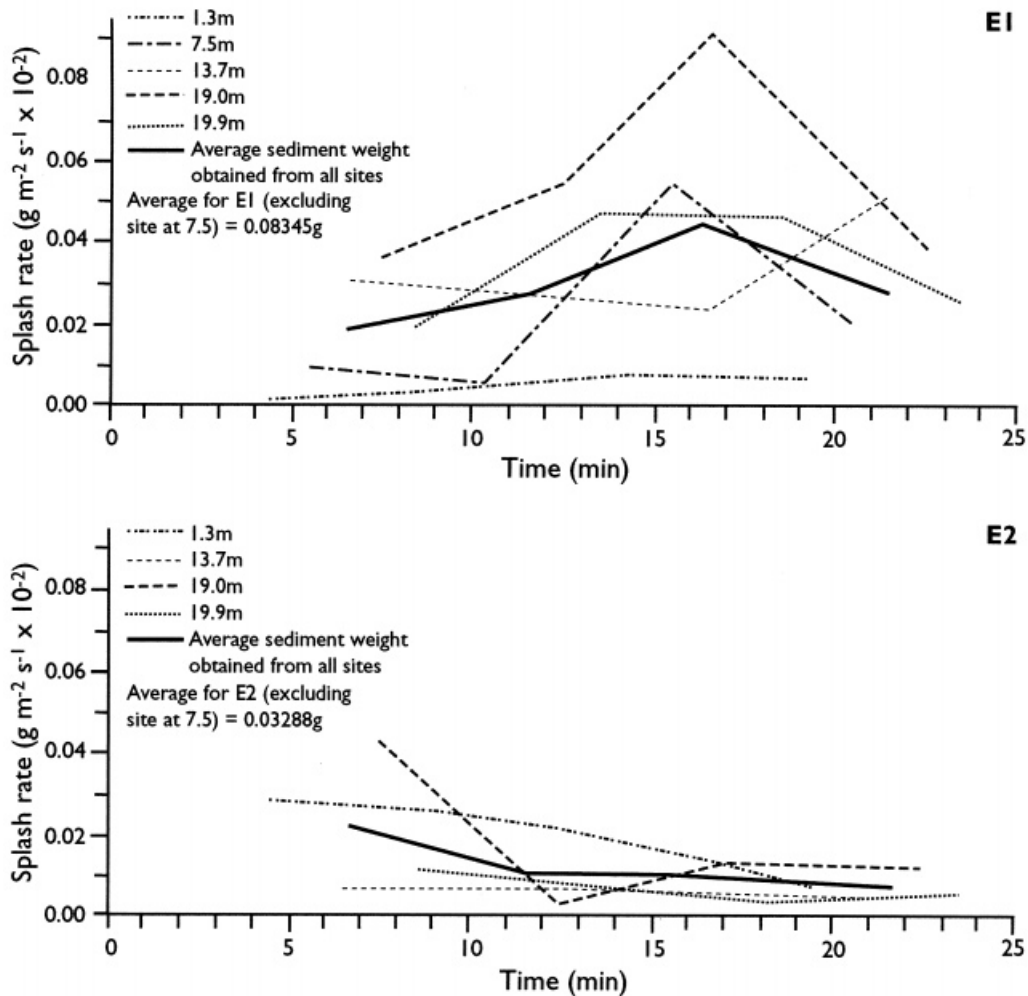
Figure 6. Splash erosion rates on the large grassland plot at Walnut Gulch (redrawn after Parsons et al. , 1994b. Modified and reprinted from Catena , 22, Parsons AJ, Abrahams AD, Wainwright J, 'Rainsplash and erosion rates in an interrill area on semi-arid grassland, southern Arizona', 215–226, 1994, with permission from Elsevier Science.)
