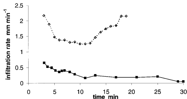
Figure 2. Examples of shrubland infiltration curves
