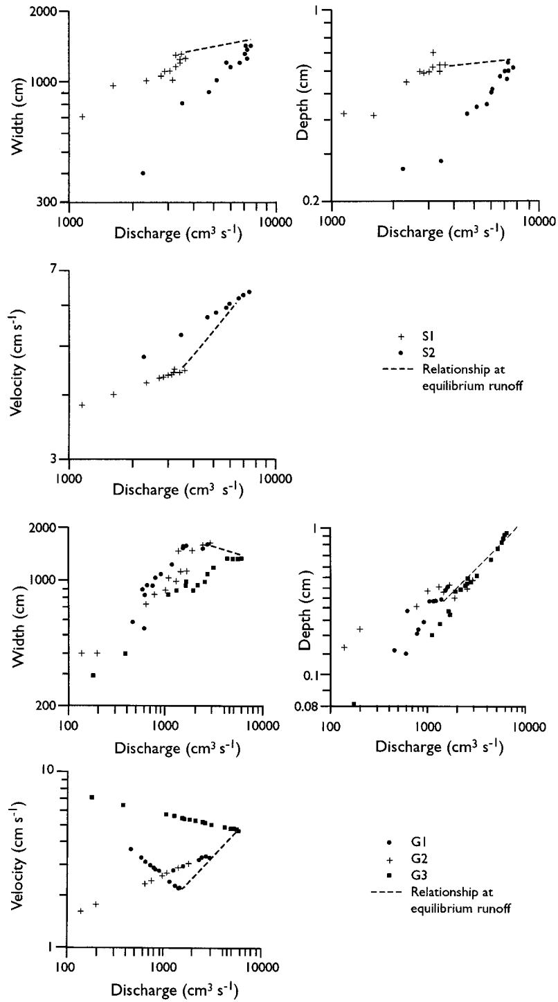
Figure 4. At-a-section hydraulic geometry relationships on the shrubland and the grassland at Walnut Gulch (redrawn after Parsons et al. , 1996b. Reproduced by permission of John Wiley & Sons Ltd.)
