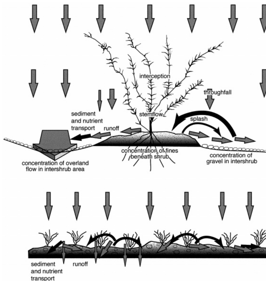
Figure 1. The basic interactions between vegetation, water movements and erosion on hillslopes, showing differences between shrub-dominated landscapes (upper) on grass-dominated landscapes (below)
