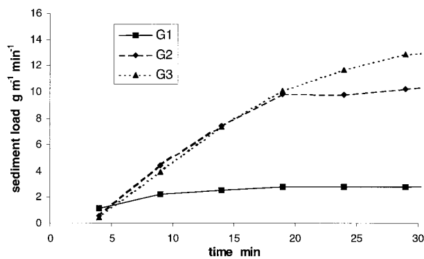
Figure 8. Sediment load at cross-sections on the large plot experiments: (a) at cross-sections 12.5 m (S1) and 21 m (S2) from the upslope boundary on the shrubland during experiments 2 and 4 (E2 and E4); and (b) at cross-sections 6 m (G1), 12 m (G2) and 20.5 m (G3) from the upslope boundary on the grassland plot during experiment 2
